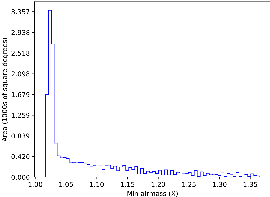
ddf_acor_sf20_lsf30_lsr50_v3.4_10yrs WFD all bands: Min airmass
