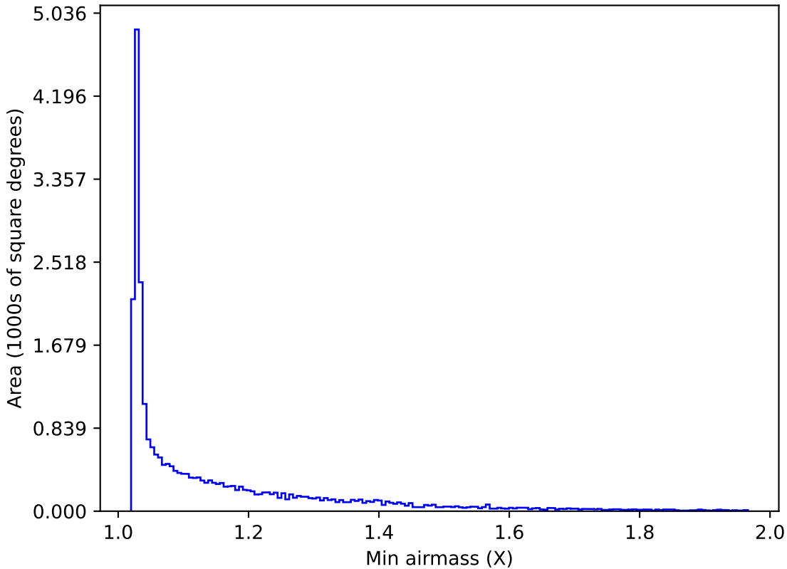
ddf_acor_sf20_lsf30_lsr50_v3.4_10yrs All sky z band: Min airmass
