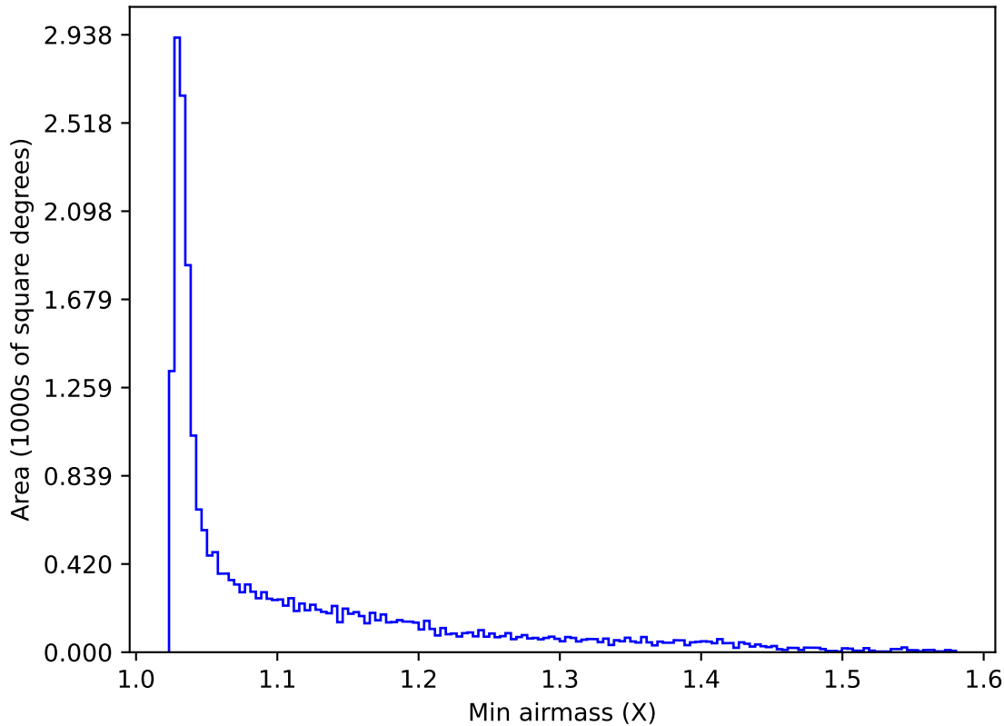
ddf_acor_sf20_lsf30_lsr50_v3.4_10yrs All sky y band: Min airmass
