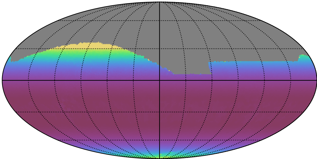
ddf_acor_sf20_lsf30_lsr50_v3.4_10yrs All sky r band: Min airmass
