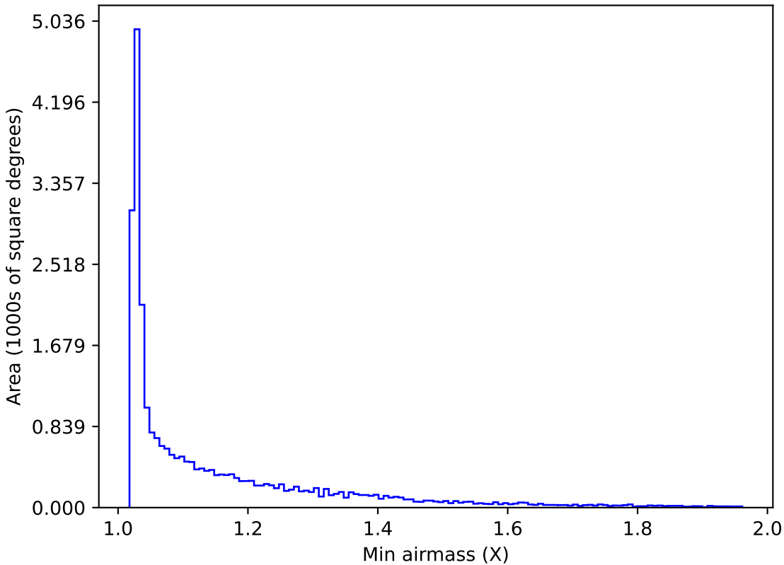
ddf_acor_sf20_lsf30_lsr50_v3.4_10yrs All sky r band: Min airmass
