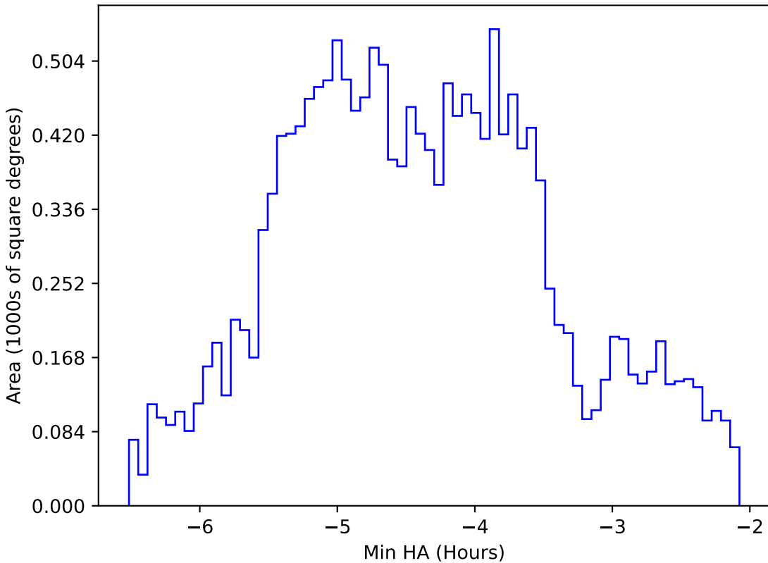
ddf_acor_sf20_lsf30_lsr50_v3.4_10yrs WFD z band: Min HA
