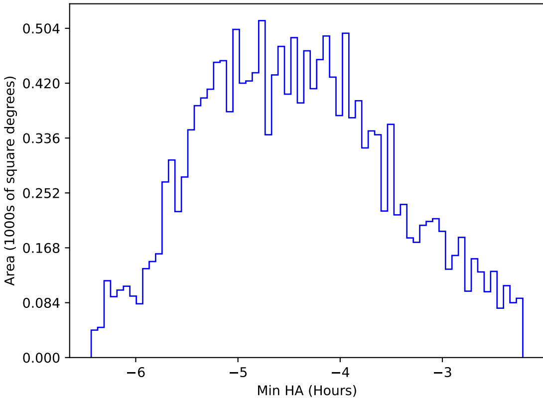
ddf_acor_sf20_lsf30_lsr50_v3.4_10yrs WFD r band: Min HA
