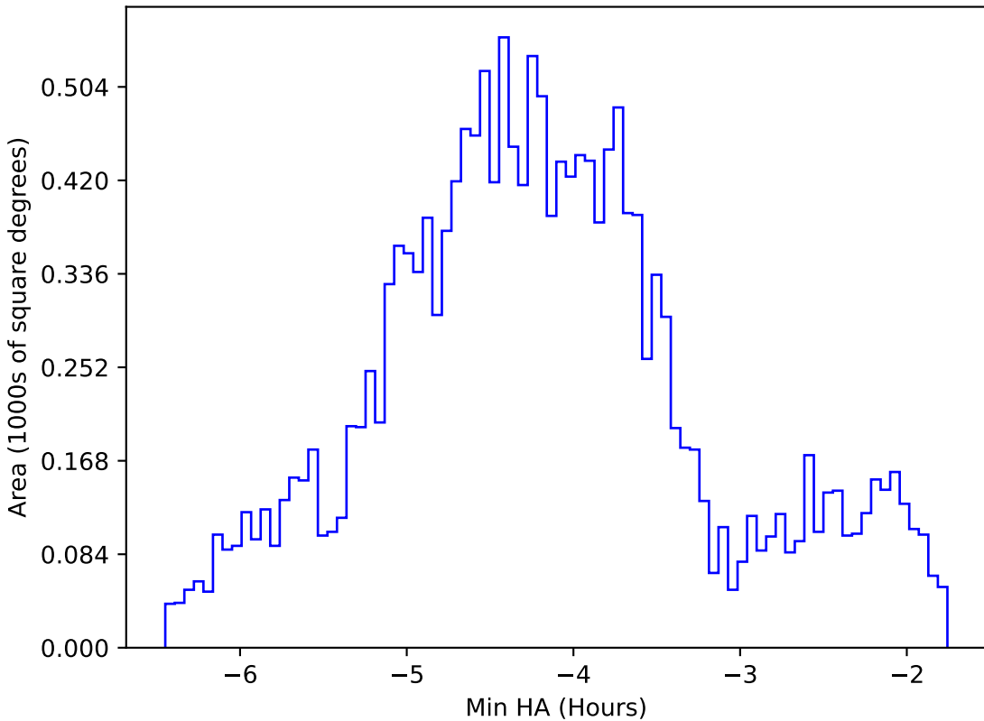
ddf_acor_sf20_lsf30_lsr50_v3.4_10yrs WFD g band: Min HA
