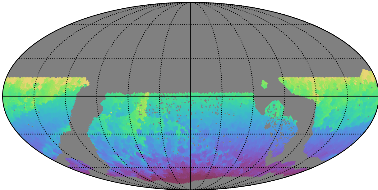
ddf_acor_sf20_lsf30_lsr50_v3.4_10yrs WFD all bands: Min HA
