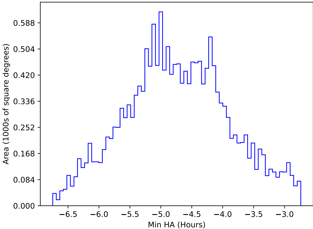
ddf_acor_sf20_lsf30_lsr50_v3.4_10yrs WFD all bands: Min HA
