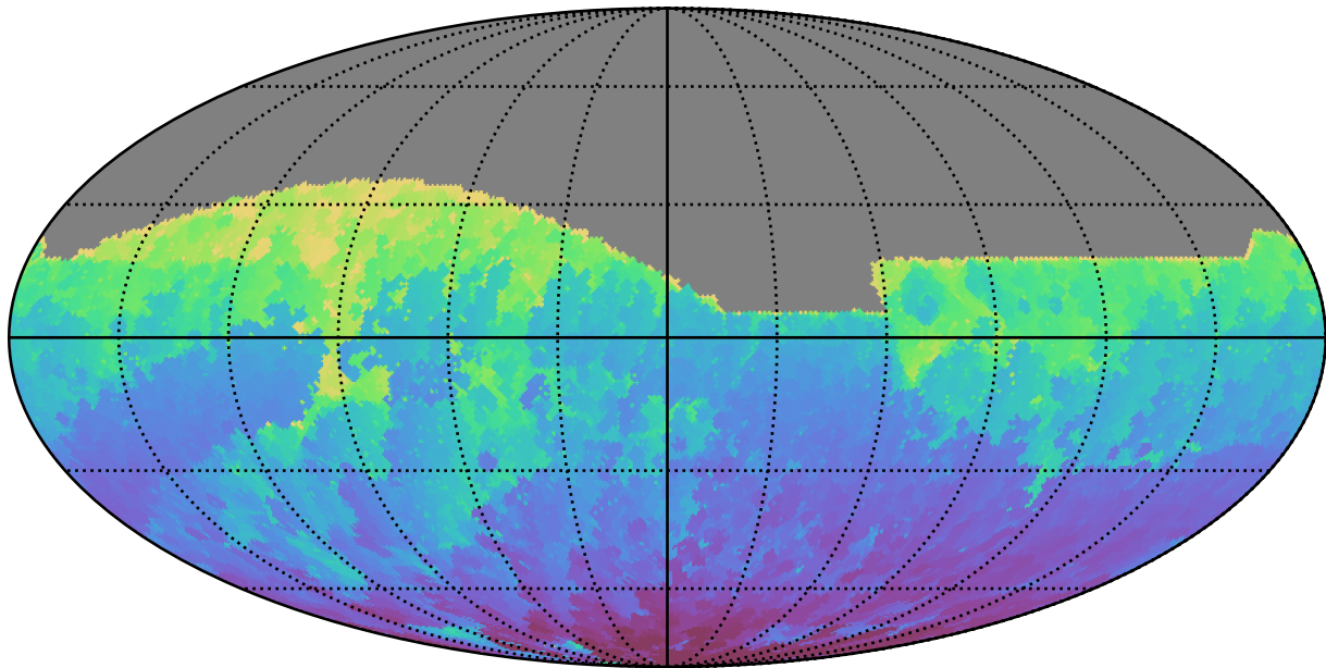
ddf_acor_sf20_lsf30_lsr50_v3.4_10yrs All sky z band: Min HA
