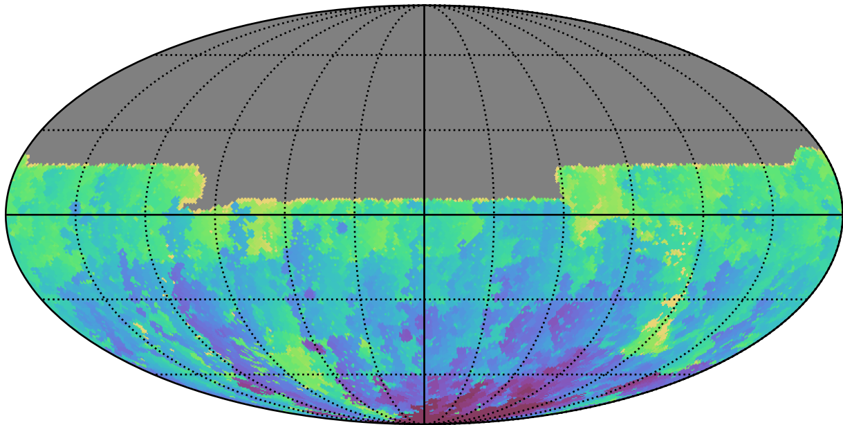
ddf_acor_sf20_lsf30_lsr50_v3.4_10yrs All sky u band: Min HA
