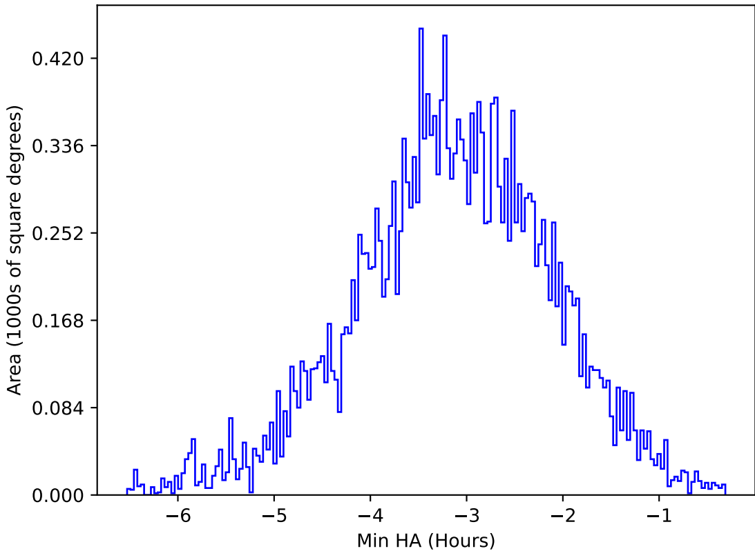
ddf_acor_sf20_ls30_lsr50_v3.4_10yrs All sky u band: Min HA
