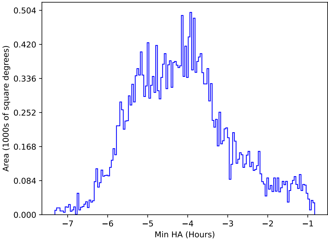
ddf_acor_sf20_ls30_lsr50_v3.4_10yrs All sky r band: Min HA
