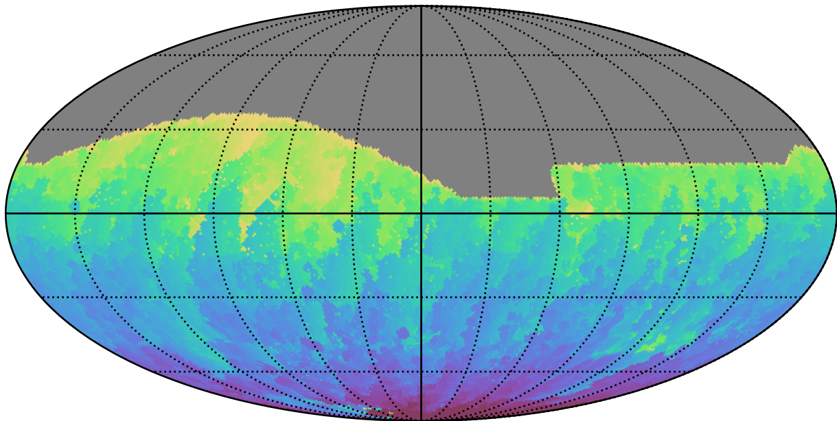
ddf_acor_sf20_lsf30_lsr50_v3.4_10yrs All sky g band: Min HA
