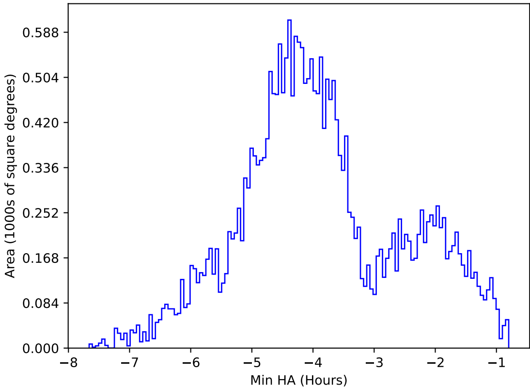
ddf_acor_sf20_ls30_lsr50_v3.4_10yrs All sky g band: Min HA
