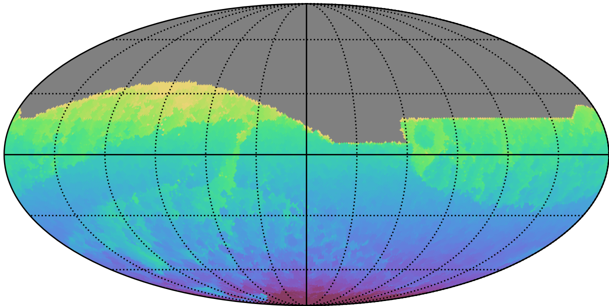
ddf_acor_sf20_lsf30_lsr50_v3.4_10yrs All sky all bands: Min HA
