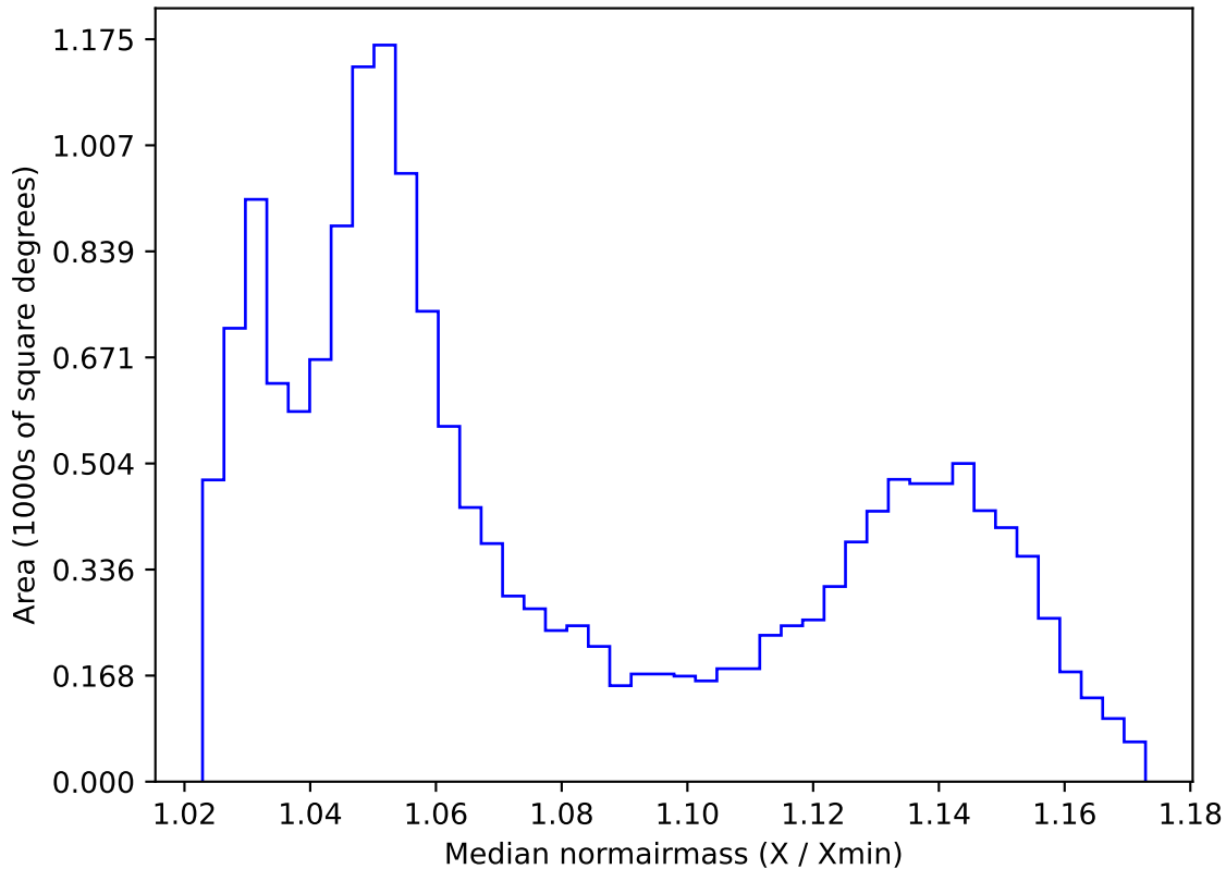
ddf_acor_sf20_lsf30_lsr50_v3.4_10yrs WFD all bands: Median normairmass
