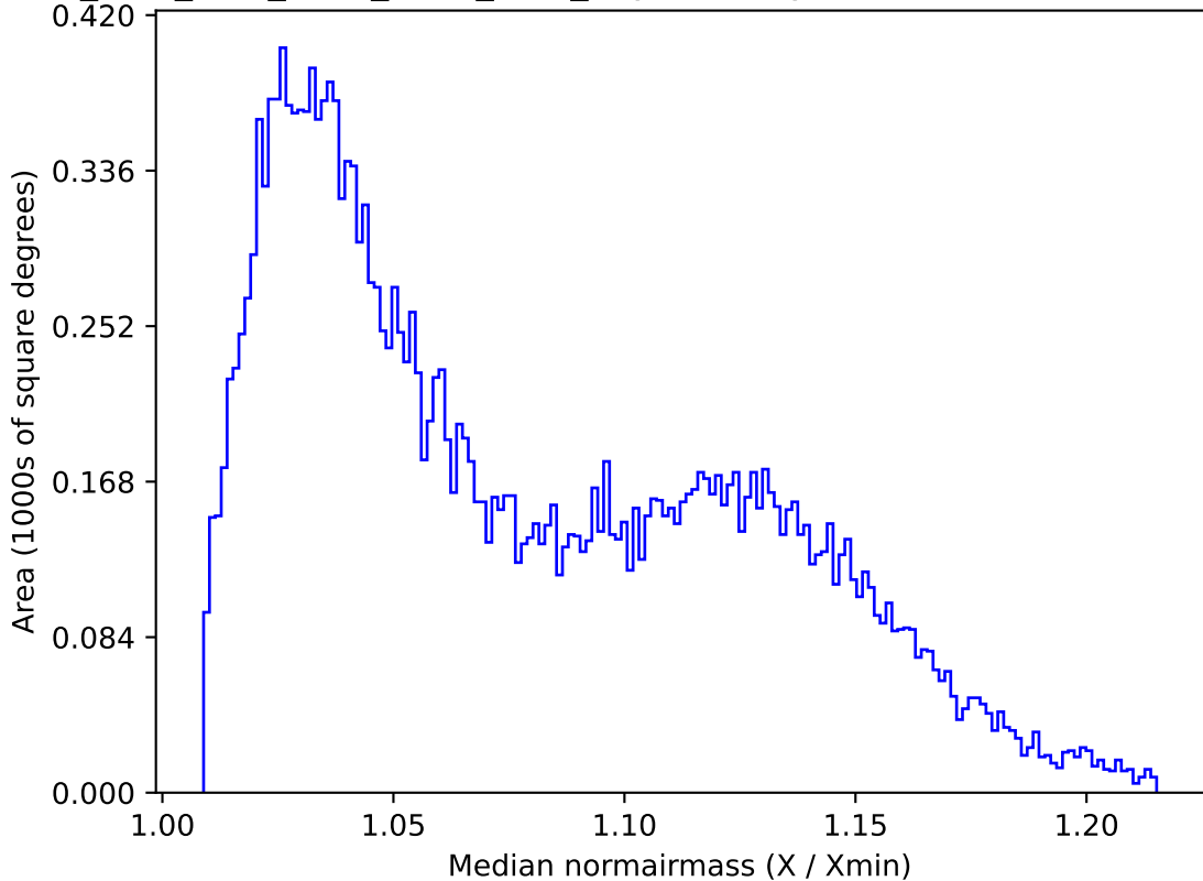
ddf_acor_sf20_lsf30_lsr50_v3.4_10yrs All sky u band: Median normairmass
