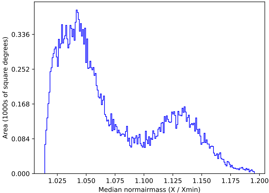
ddf_acor_sf20_lsf30_lsr50_v3.4_10yrs All sky r band: Median normairmass
