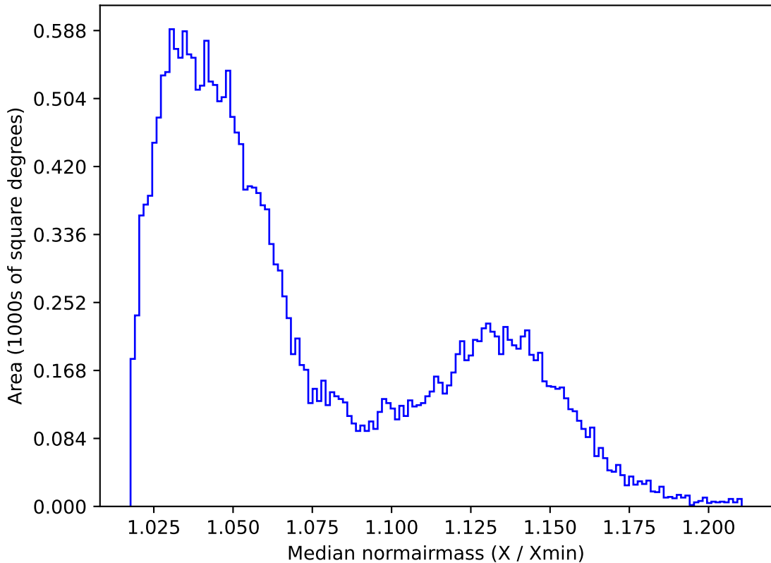
ddf_acor_sf20_lsf30_lsr50_v3.4_10yrs All sky i band: Median normairmass
