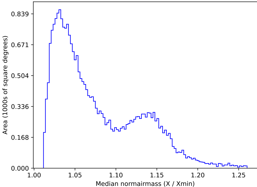
ddf_acor_sf20_lsf30_lsr50_v3.4_10yrs All sky g band: Median normairmass
