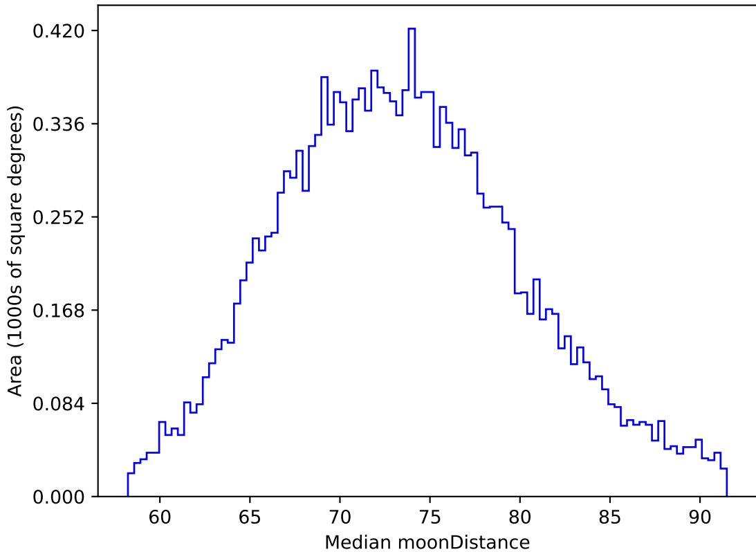
ddf_acor_sf20_lsf30_lsr50_v3.4_10yrs WFD z band: Median moonDistance
