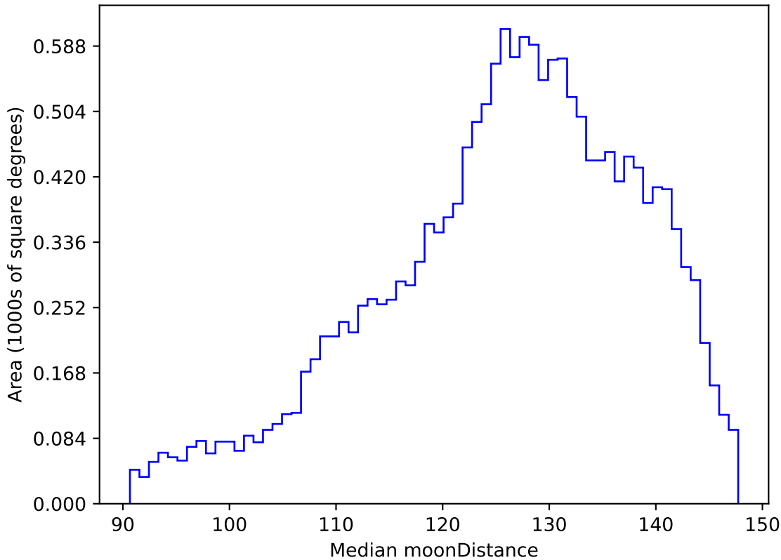
ddf_acor_sf20_lsf30_lsr50_v3.4_10yrs WFD u band: Median moonDistance
