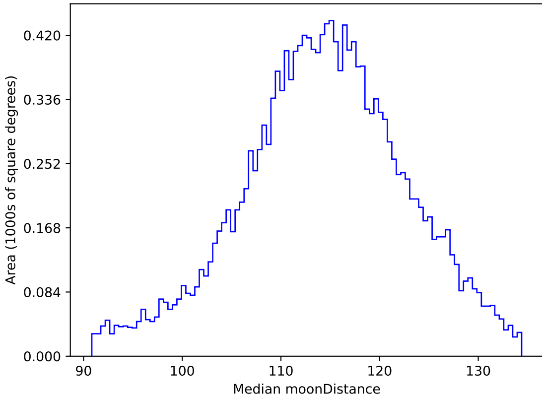
ddf_acor_sf20_lsf30_lsr50_v3.4_10yrs WFD g band: Median moonDistance
