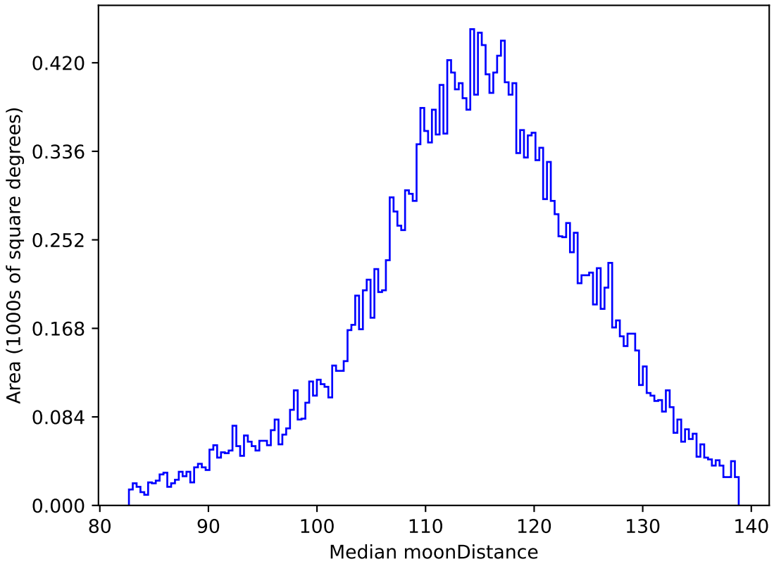
ddf_acor_sf20_lsf30_lsr50_v3.4_10yrs All sky g band: Median moonDistance
