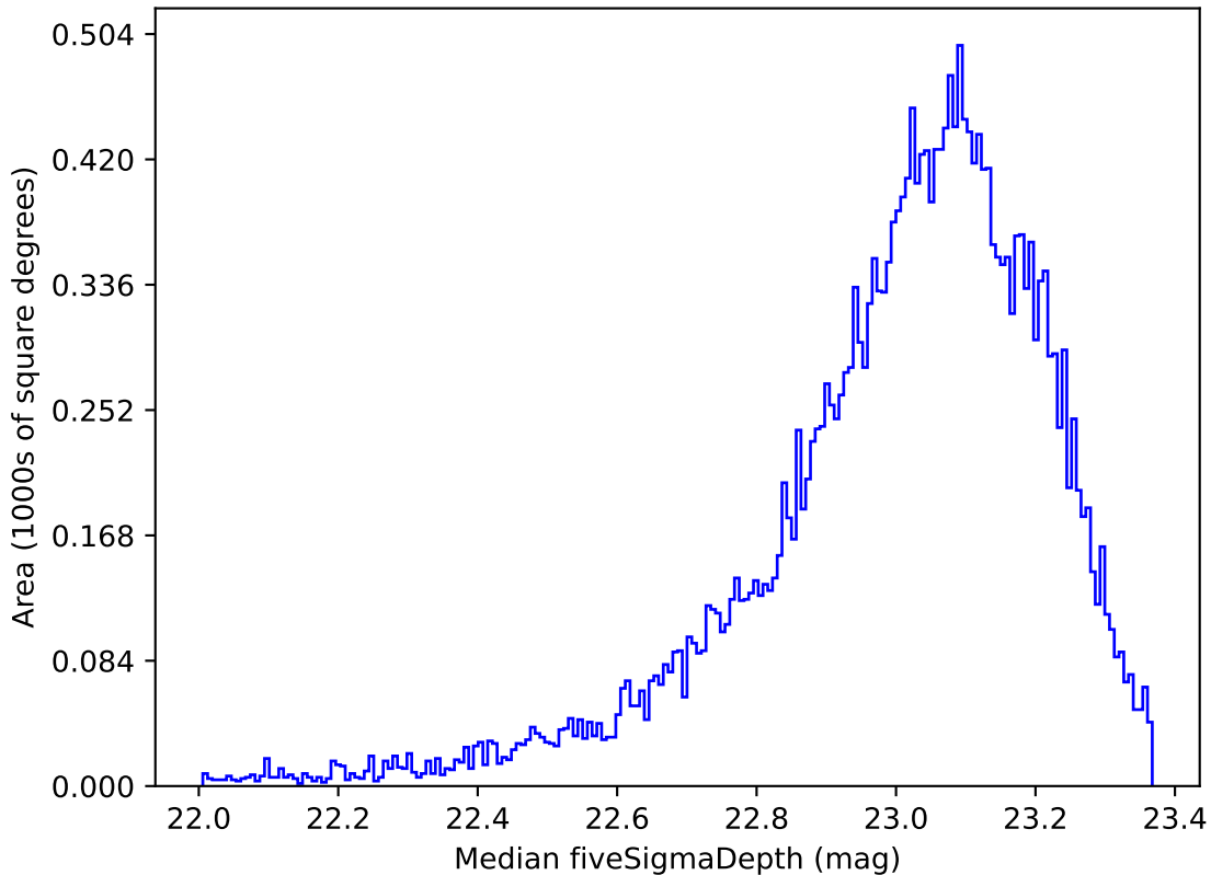
ddf_acor_sf20_lsf30_lsr50_v3.4_10yrs Yr 1 z band: Median fiveSigmaDepth
