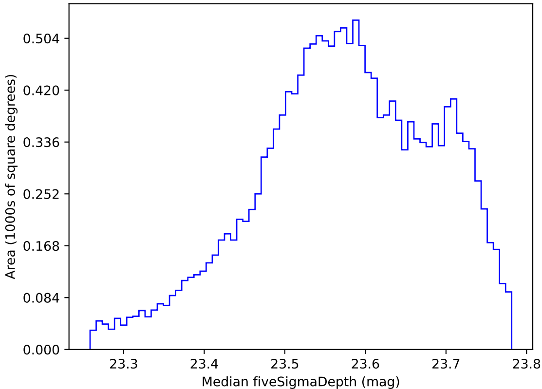
ddf_acor_sf20_lsf30_lsr50_v3.4_10yrs WFD i band: Median fiveSigmaDepth
