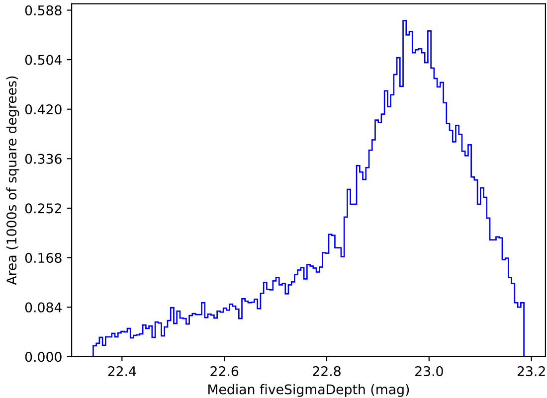
ddf_acor_sf20_lsf30_lsr50_v3.4_10yrs All sky z band: Median fiveSigmaDepth
