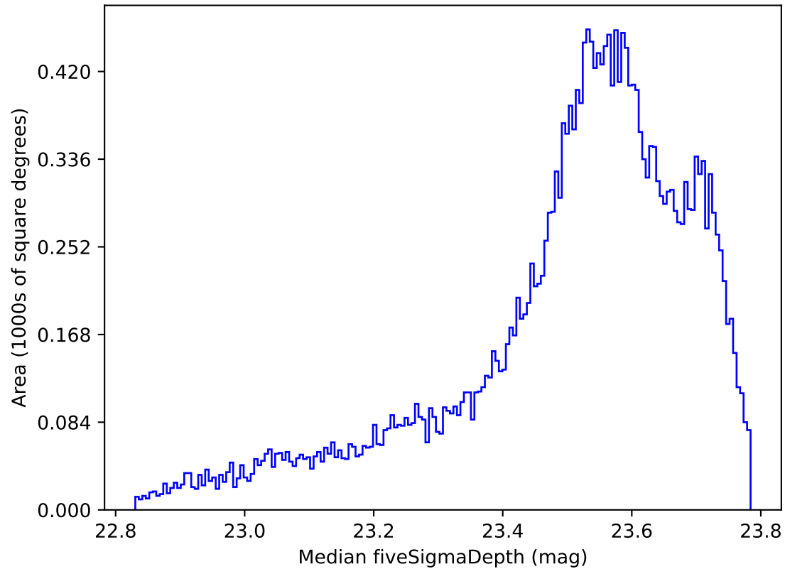
ddf_acor_sf20_lsf30_lsr50_v3.4_10yrs All sky i band: Median fiveSigmaDepth
