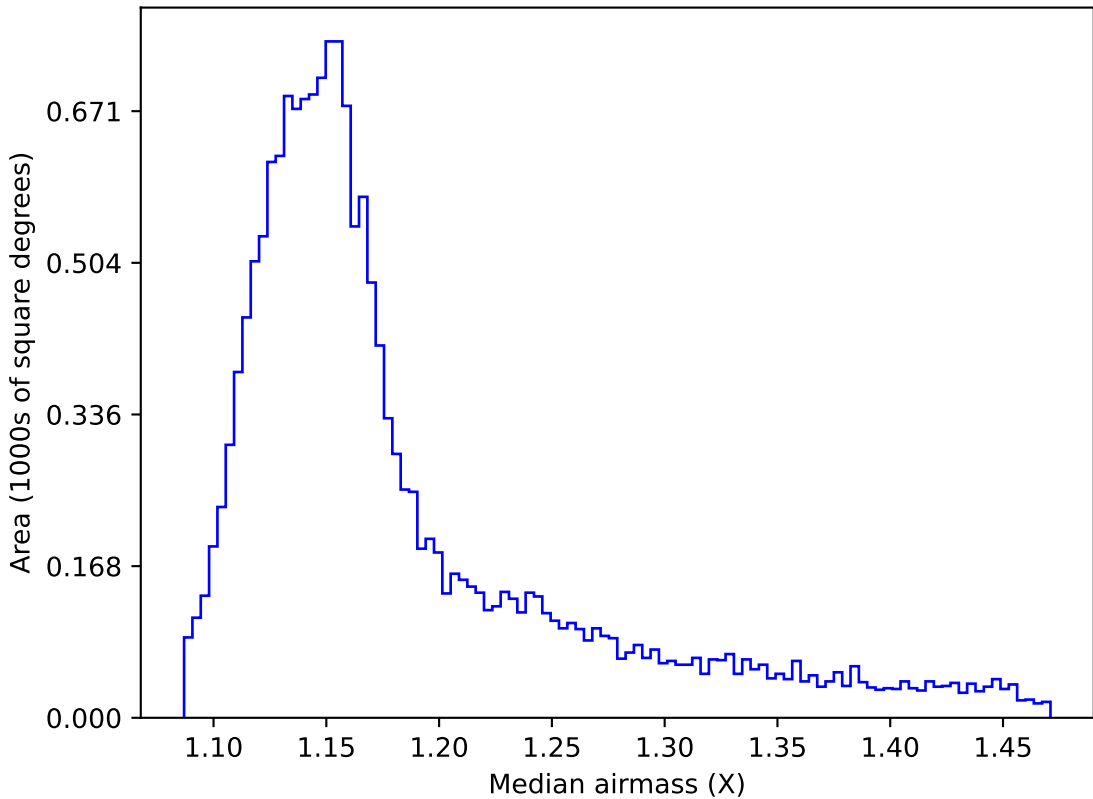
ddf_acor_sf20_lsf30_lsr50_v3.4_10yrs WFD z band: Median airmass
