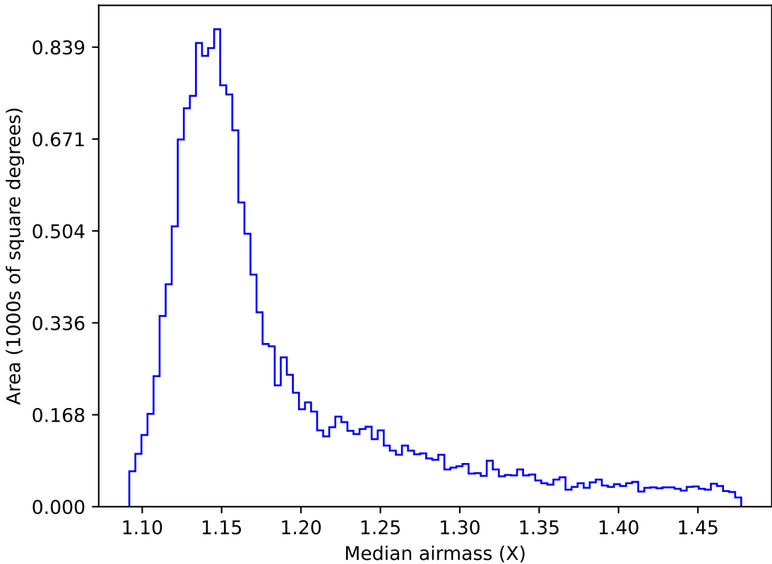
ddf_acor_sf20_lsf30_lsr50_v3.4_10yrs WFD y band: Median airmass
