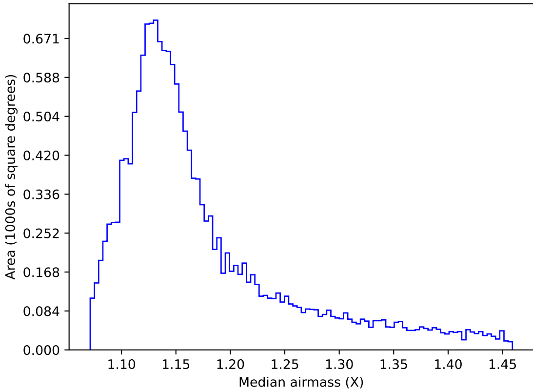
ddf_acor_sf20_lsf30_lsr50_v3.4_10yrs WFD u band: Median airmass
