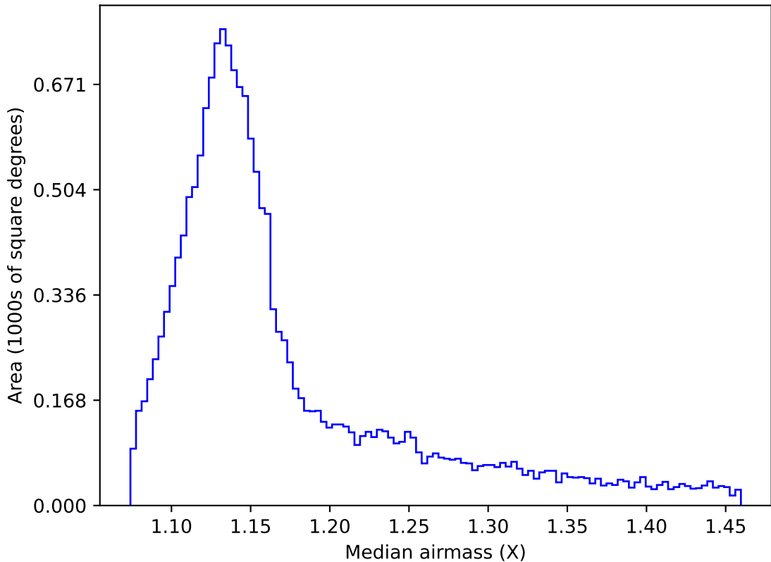
ddf_acor_sf20_lsf30_lsr50_v3.4_10yrs WFD r band: Median airmass
