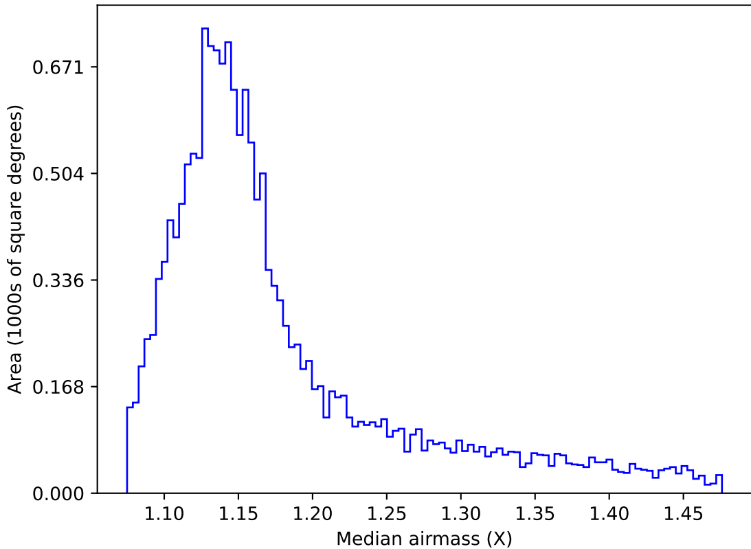
ddf_acor_sf20_lsf30_lsr50_v3.4_10yrs WFD g band: Median airmass
