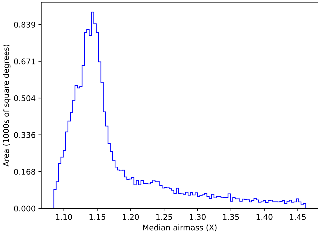
ddf_acor_sf20_lsf30_lsr50_v3.4_10yrs WFD all bands: Median airmass
