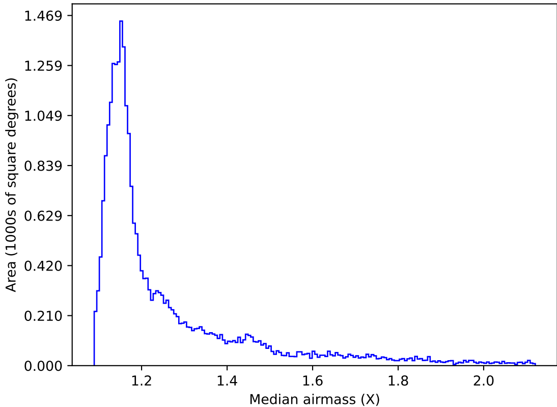
ddf_acor_sf20_lsf30_lsr50_v3.4_10yrs All sky z band: Median airmass
