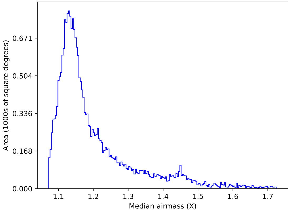
ddf_acor_sf20_lsf30_lsr50_v3.4_10yrs All sky u band: Median airmass
