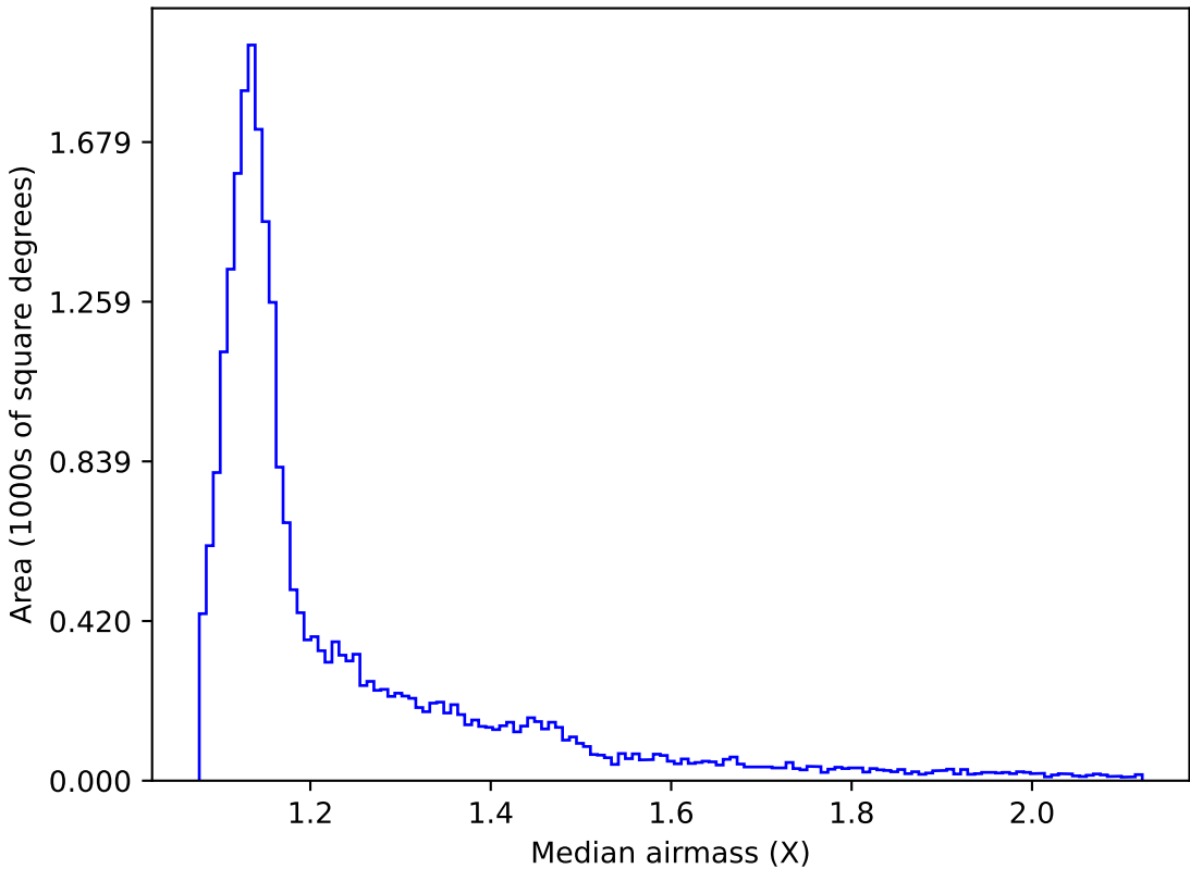
ddf_acor_sf20_lsf30_lsr50_v3.4_10yrs All sky r band: Median airmass
