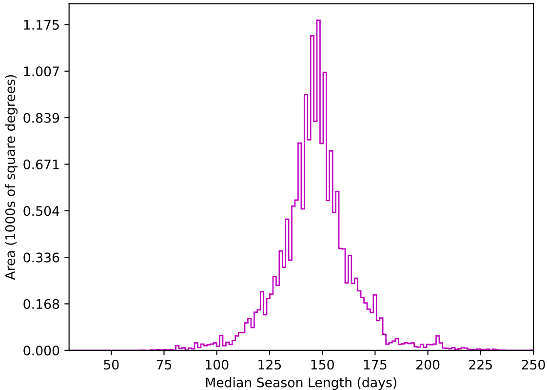
ddf_acor_sf20_lsf30_lsr50_v3.4_10yrs WFD z band: Median Season Length
