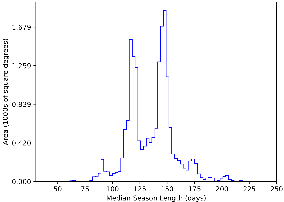
ddf_acor_sf20_lsf30_lsr50_v3.4_10yrs WFD y band: Median Season Length
