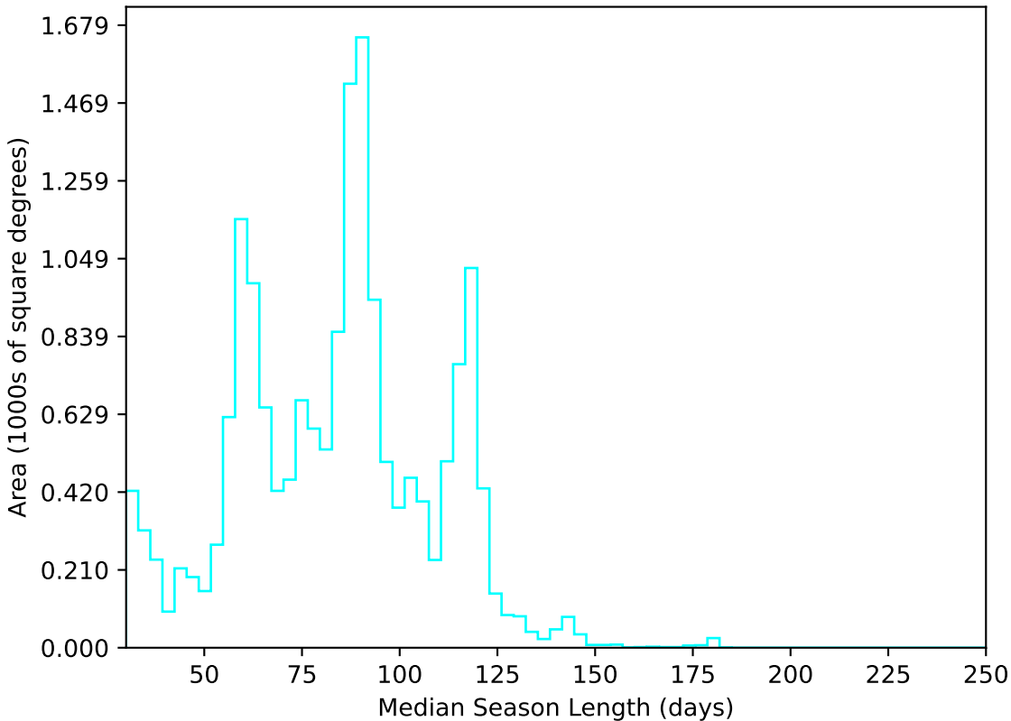
ddf_acor_sf20_ls30_lsr50_v3.4_10yrs WFD u band: Median Season Length
