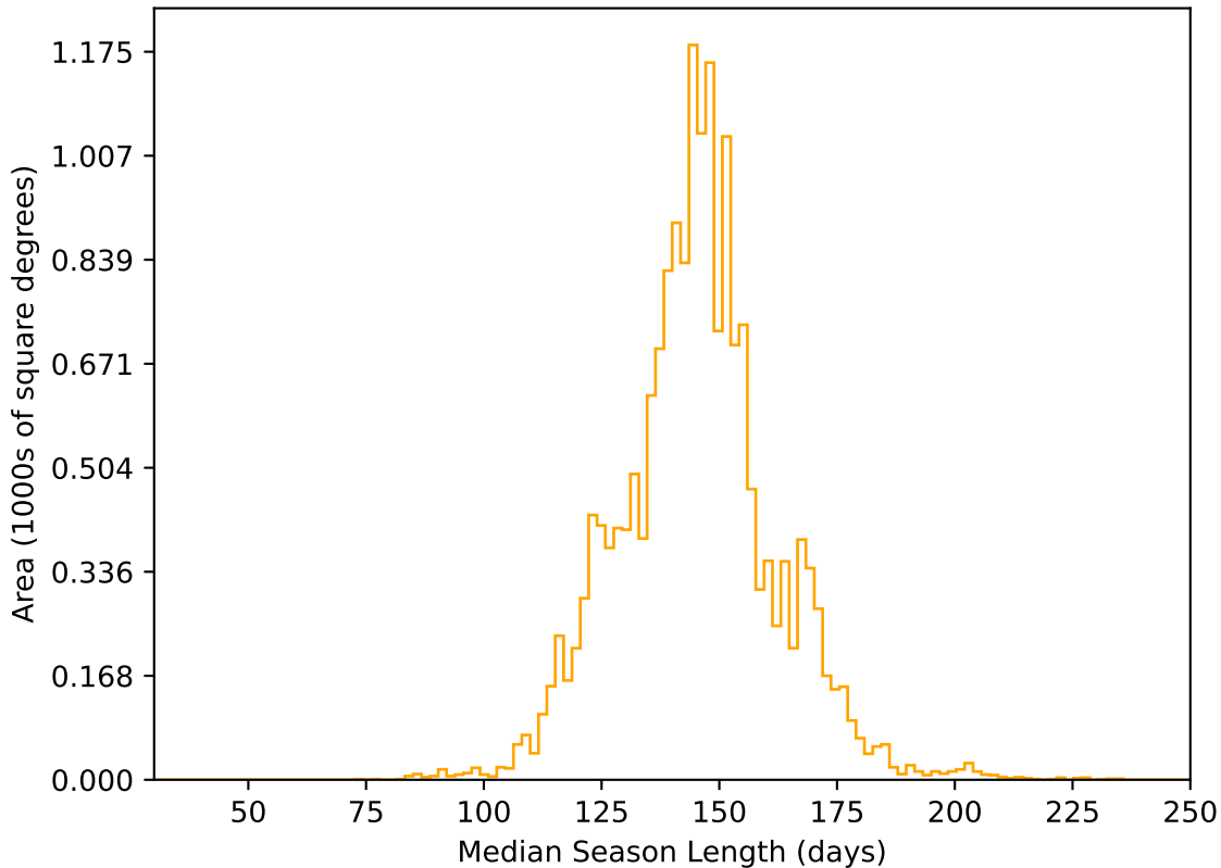
ddf_acor_sf20_lsf30_lsr50_v3.4_10yrs WFD r band: Median Season Length
