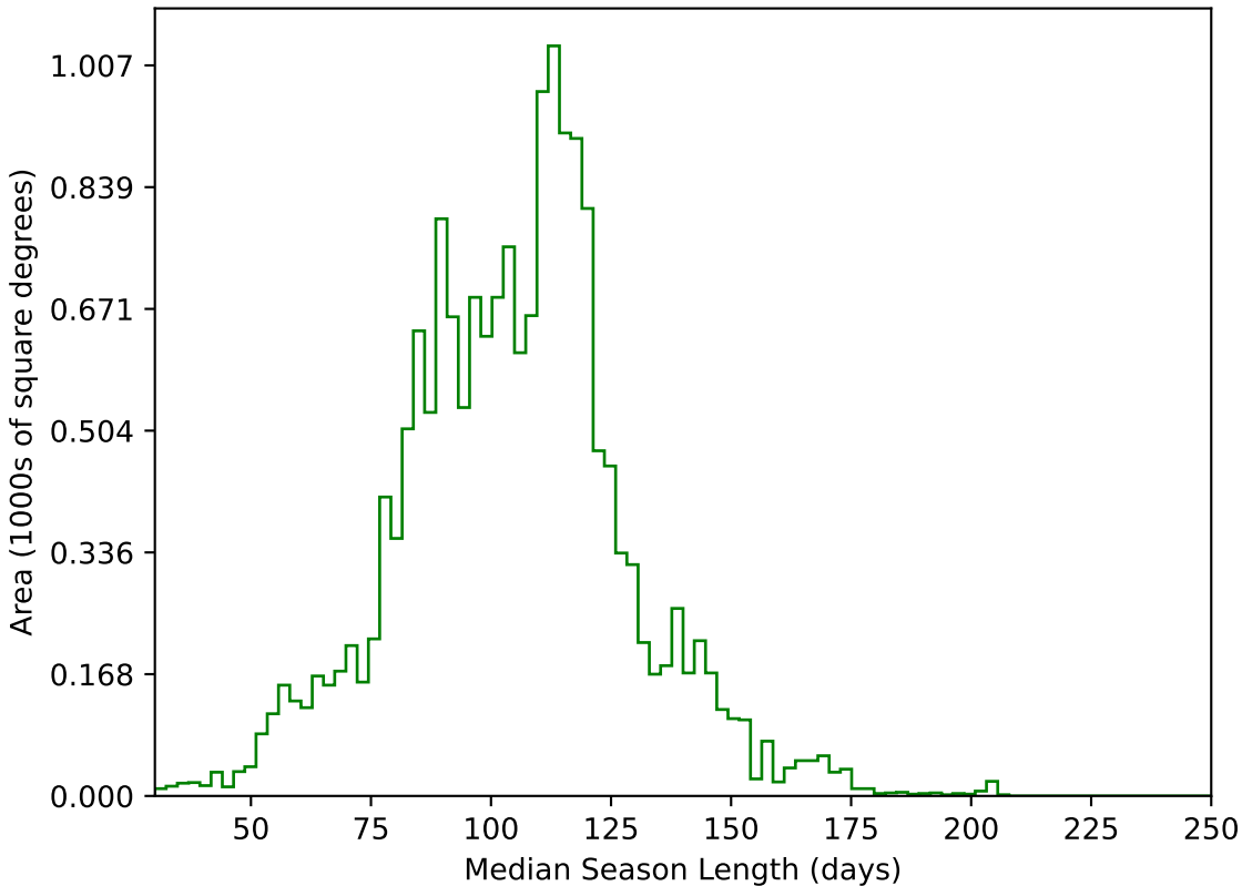
ddf_acor_sf20_lsf30_lsr50_v3.4_10yrs WFD g band: Median Season Length
