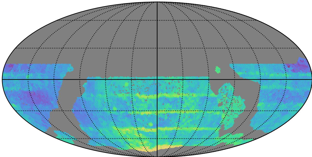
ddf_acor_sf20_lsf30_lsr50_v3.4_10yrs WFD all bands: Median Season Length
