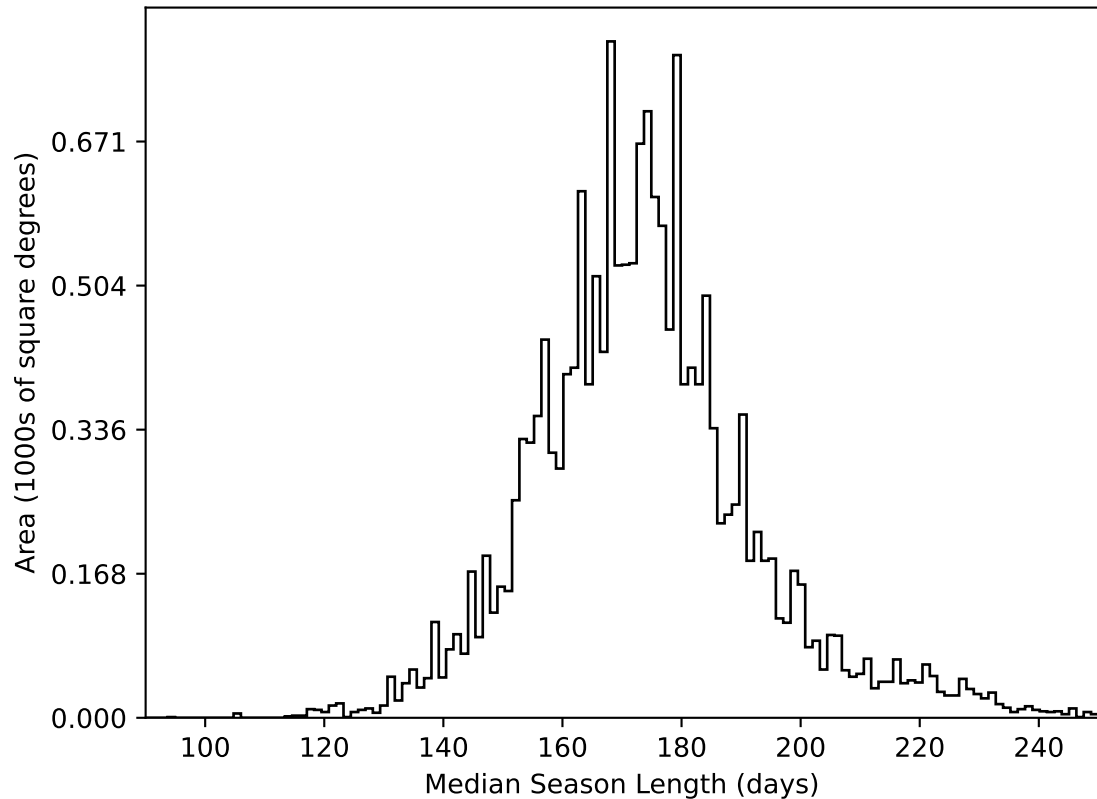
ddf_acor_sf20_lsf30_lsr50_v3.4_10yrs WFD all bands: Median Season Length
