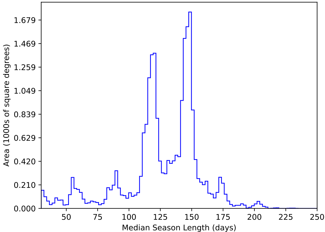
ddf_acor_sf20_lsf30_lsr50_v3.4_10yrs All sky y band: Median Season Length
