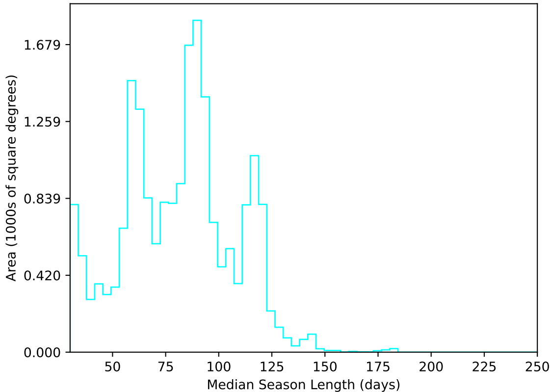
ddf_acor_sf20_lsf30_lsr50_v3.4_10yrs All sky u band: Median Season Length
