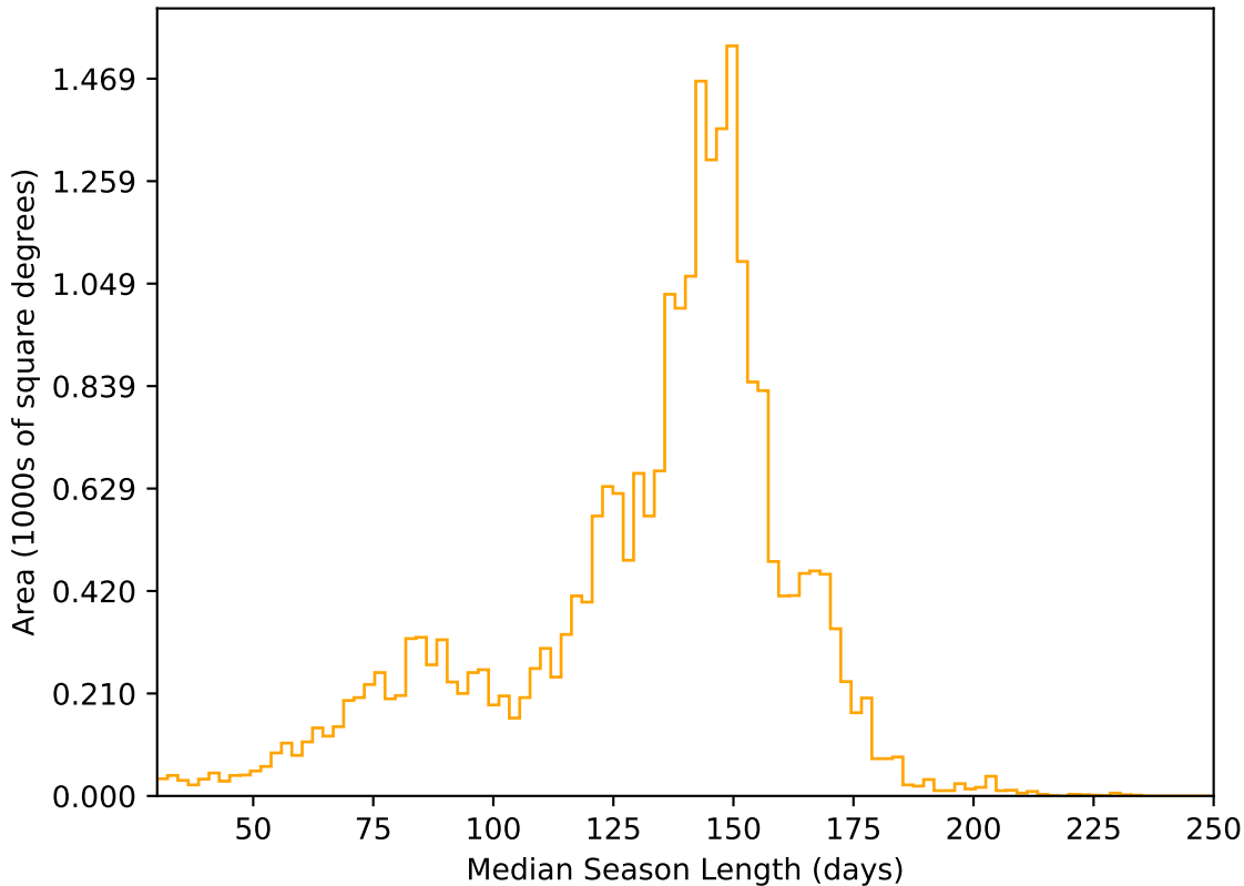
ddf_acor_sf20_lsf30_lsr50_v3.4_10yrs All sky r band: Median Season Length
