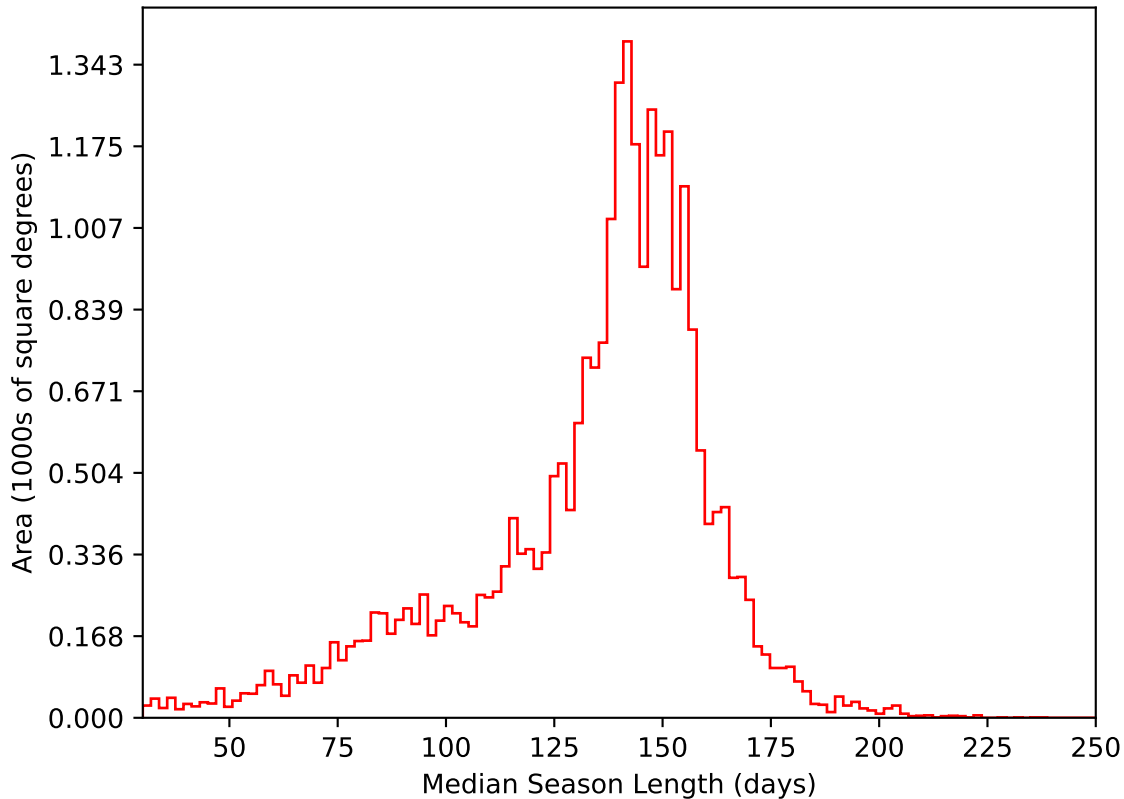
ddf_acor_sf20_lsf30_lsr50_v3.4_10yrs All sky i band: Median Season Length
